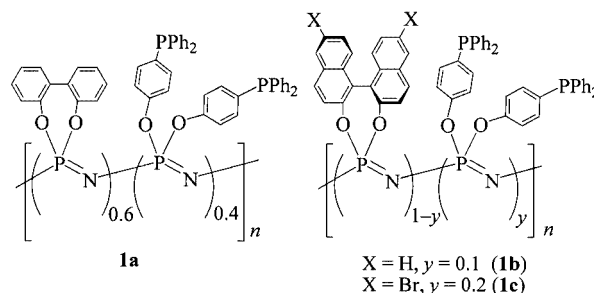
Scheme 1. Polyphosphazenes 1a , 1b , 1c
