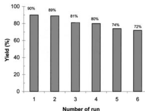
Figure 1. Transfer hydrogenation of acetophenone by 2a ; conditions: reaction carried out at 82 °C using 5 mmol of acetophenone (0.25 M in propan-2-ol); ketone/Ru/NaOH = 500:1:24; yield of 1-phenylethanol after 24 h determined by GC; global TON for six uses = 2430
